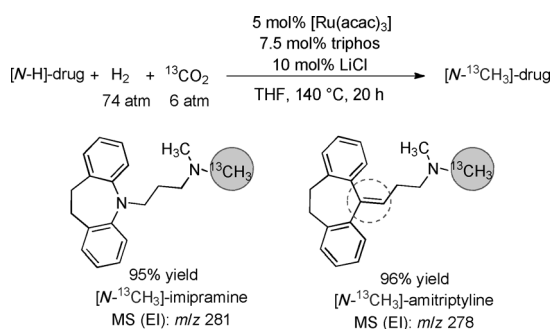
Scheme 5. Direct synthesis of [N- 13 CH 3 ]drugs from 13 CO 2 .
